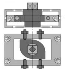
Bottom flanged external limit Stops open/close for sizes 205 - H15
